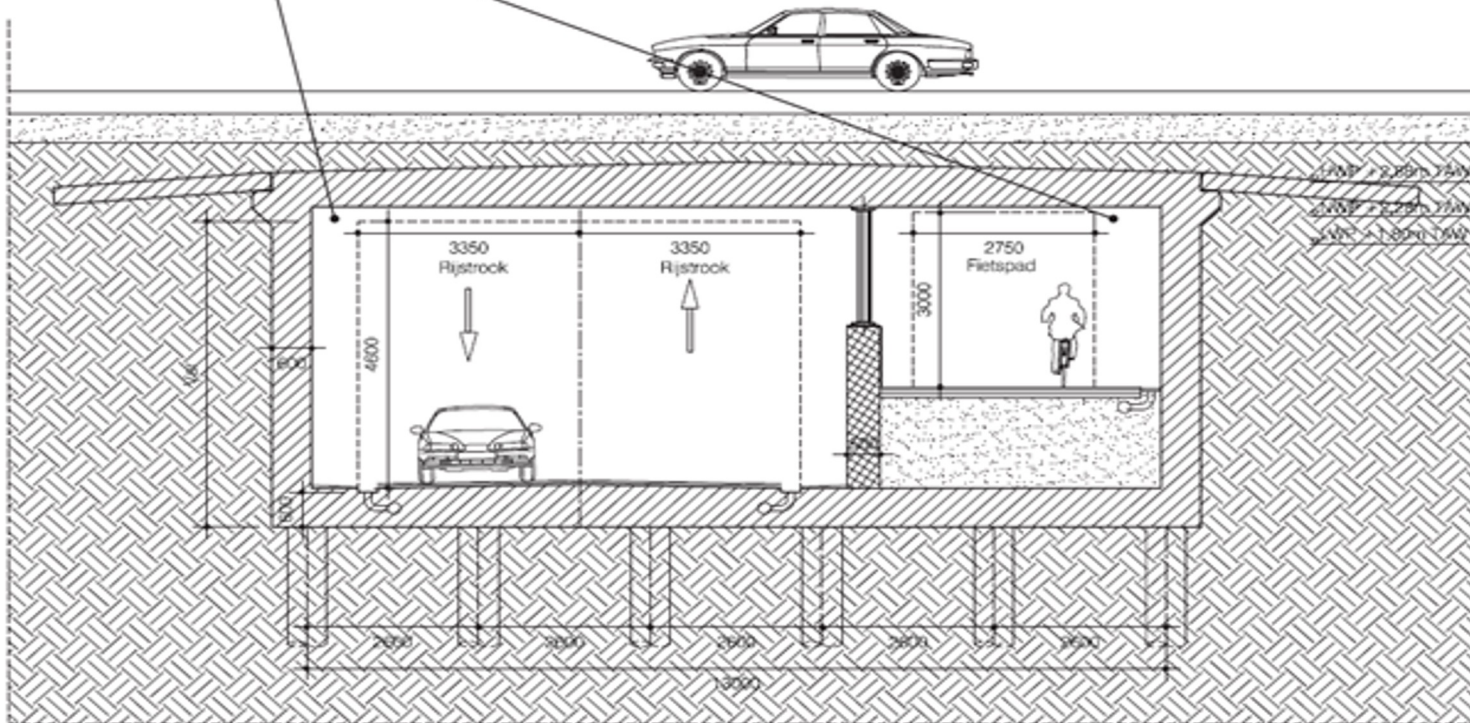
Dwarsdoorsnede tunnel
